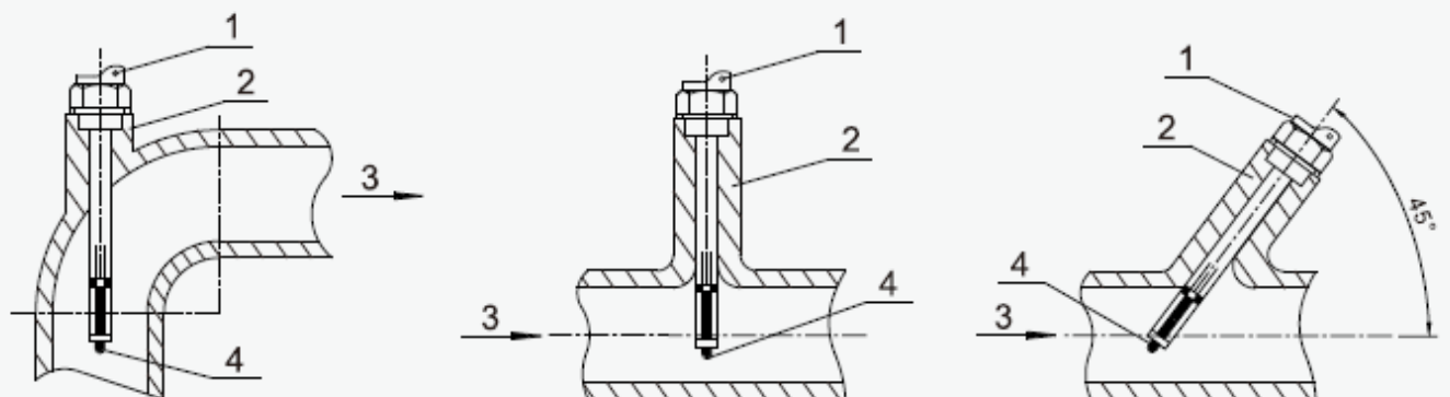
1-Temperature sensor sheath ; 2-Welding base ; 3-Fluid direction ; 4-Temperature sensor probe
